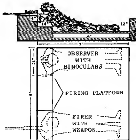
Figure 4-9. Expedient position.
